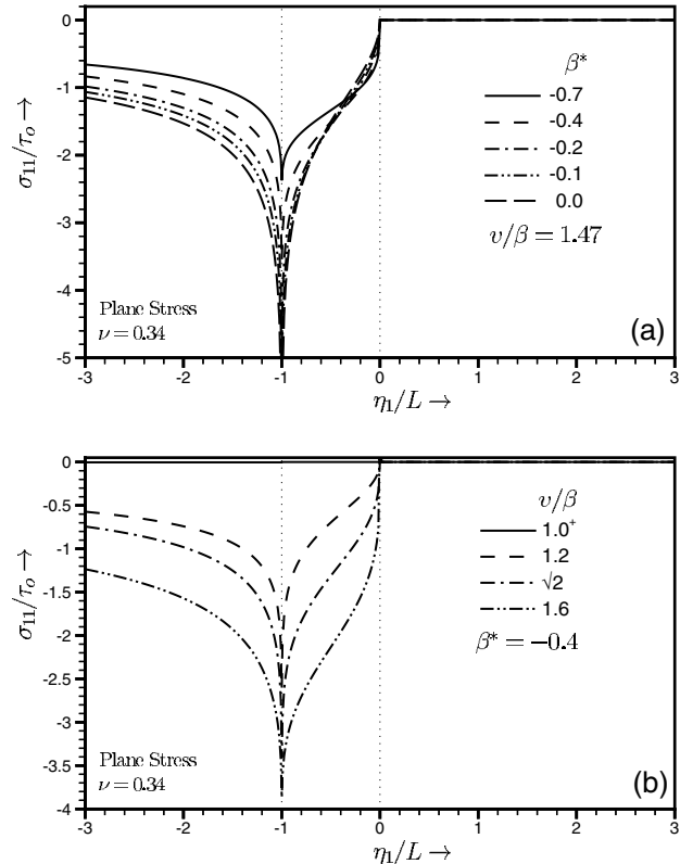
Figure 11. Intersonically propagating mode II crack with a velocity weakening cohesive zone. (a) Stress component \sigma_{11} on the crack plane for v/\beta = 1.47 and for different values of the weakening parameter \beta^* . (b) Stress component \sigma_{11} on the crack plane for \beta^* = -0.4 and for different values of crack tip speed v .
